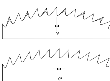
Tooth shapes F and C
