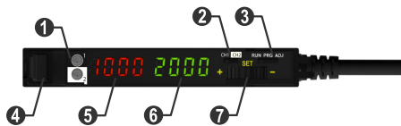
Figure 1. DF-G3 IO Link Model Features
