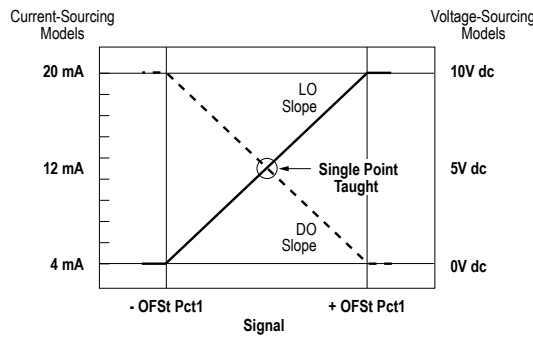
Figure 3. One-Point SET (Light Operate shown)
