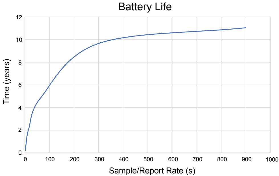
Battery life by sample/report rate (s)
