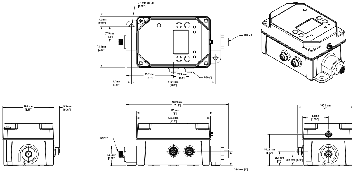
DXM1200E dimensions
