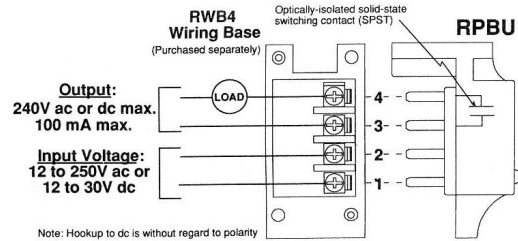
Figure 14. RPBU—Wiring Diagram
