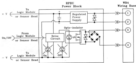
Figure 13. RPBU—Schematic
