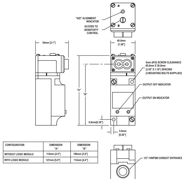
Figure 19. Dimensions for the fiber models
