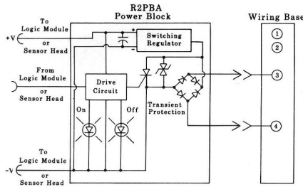
Figure 7. R2PBA & R2PBB—Schematic
