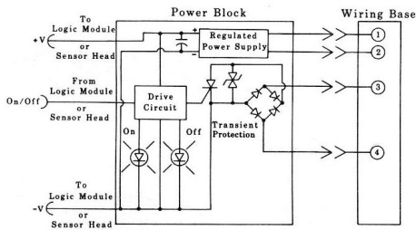
Figure 3. RPBA & RPBA-1—Schematic
