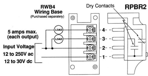
Figure 12. RPBR2—Wiring Diagram
