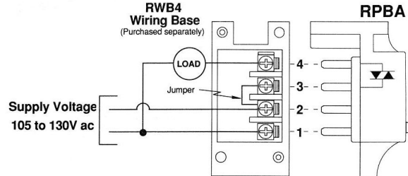
Figure 4. RPBA & RPBA-1—Wiring Diagram
