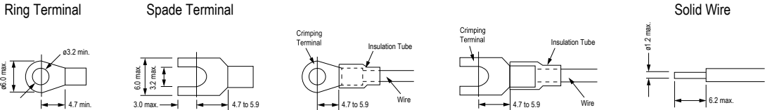
Applicable Crimping Terminal
