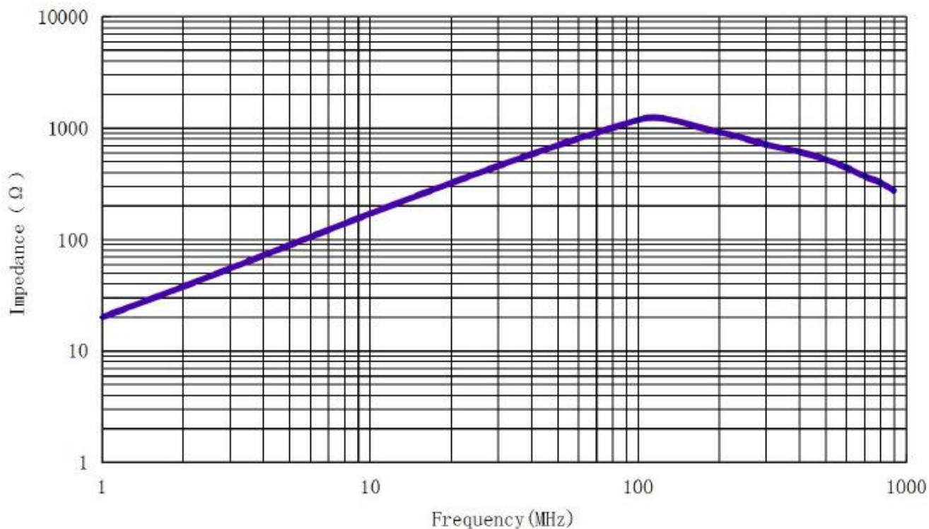
Impedance (Ω) VS Frequency (MHz)
