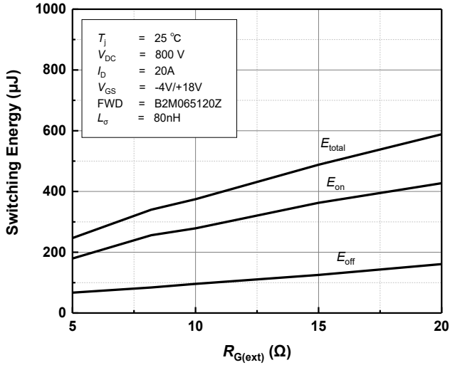
Figure 21 Clamped Inductive Switching Energy vs. External Gate Resistance at T j =25°C
