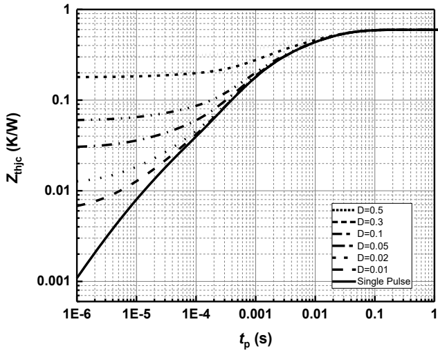
Figure 25 Transient Thermal Impedance (Junction - Case)
