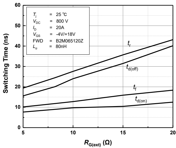
Figure 23 Clamped Inductive Switching Time vs. External Gate Resistance at T j =25°C
