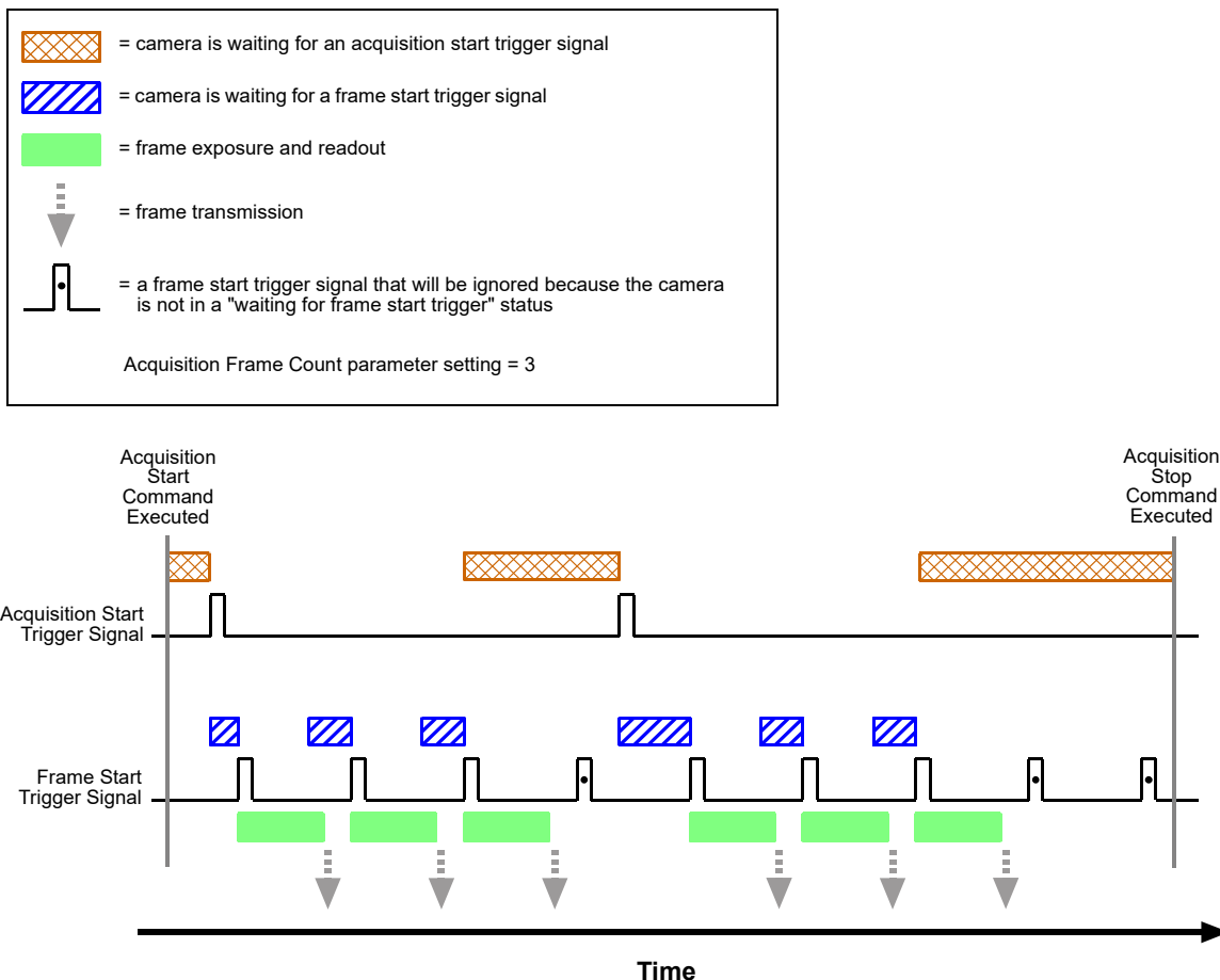
Fig. 30: Acquisition Start and Frame Start Triggering
