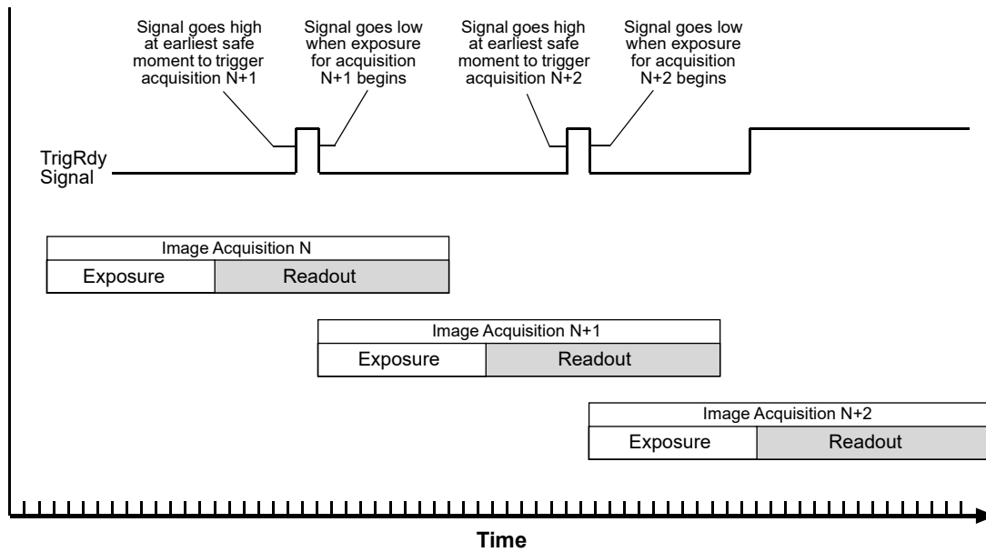
Fig. 47: Trigger Ready Signal
