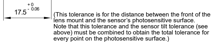
Fig. 12: Sensor Positioning Accuracy for Cameras With 90° Head Housing (in mm unless otherwise noted)
