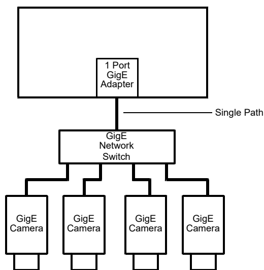
Fig. 17: Multiple Cameras on a Network
