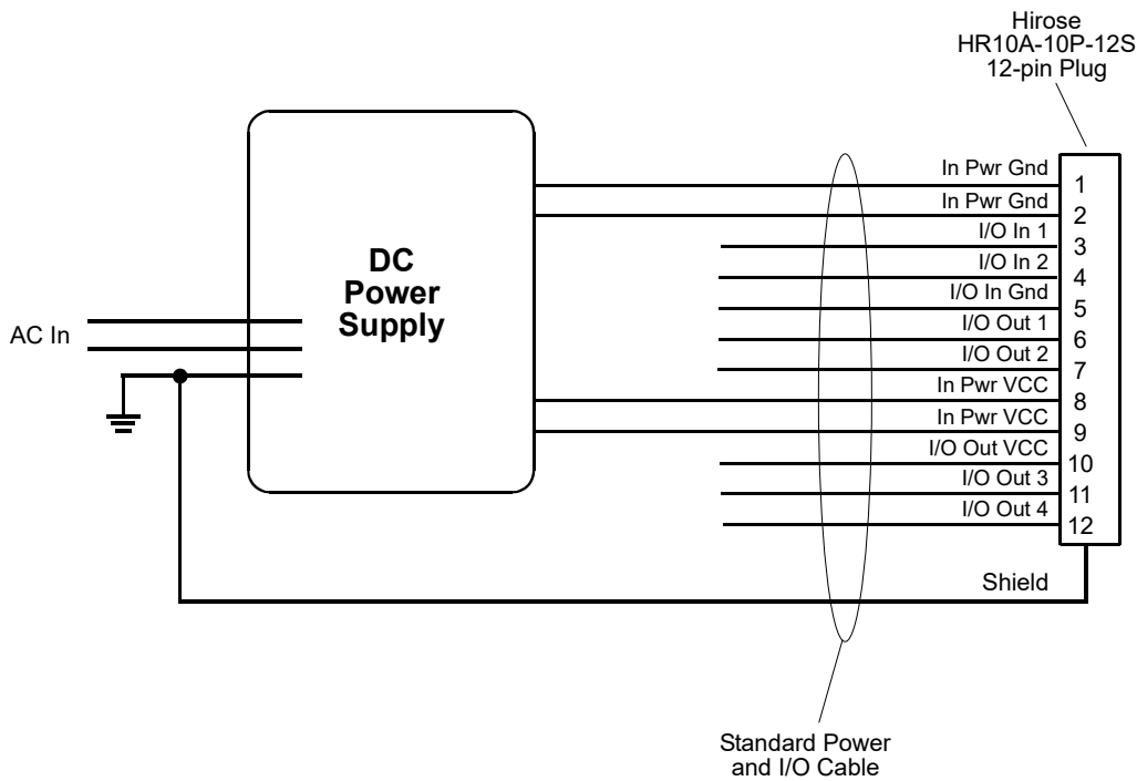
Fig. 22: Standard Power and I/O Cable
