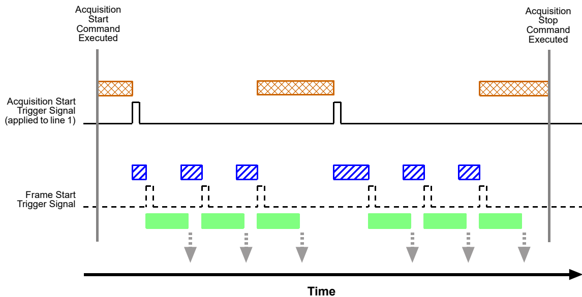
Fig. 42: Use Case 3 - Acquisition Start Trigger On and Frame Start Trigger Off
