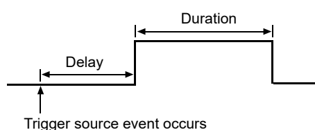
Fig. 28: Timer Signal
