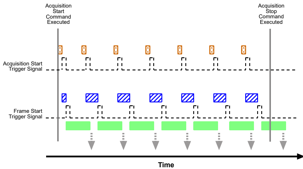
Fig. 40: Use Case 1 - Acquisition Start Trigger Off and Frame Start Trigger Off
