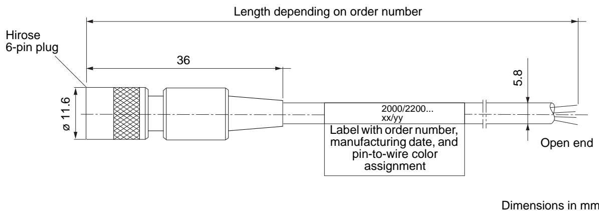
Fig. 1: Cable Overview
