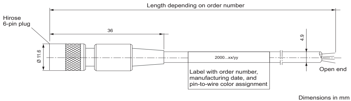
Fig. 1: Cable Overview
