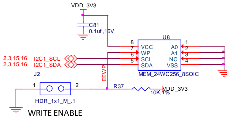
Figure 54. EEPROM Circuitry
