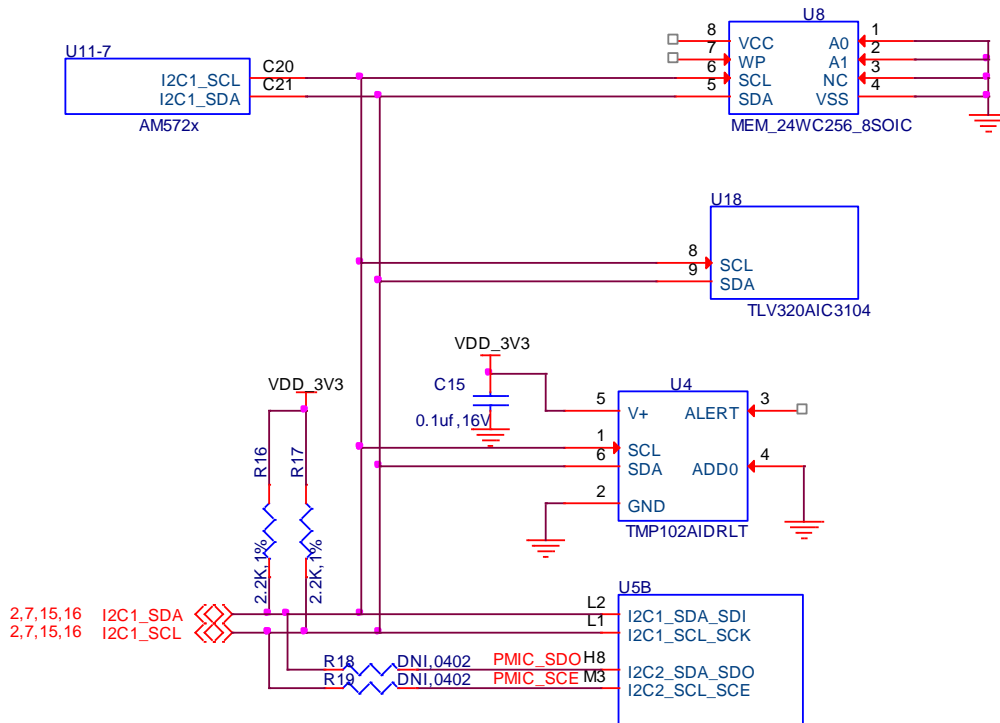
Figure 57. I2C1 Bus
