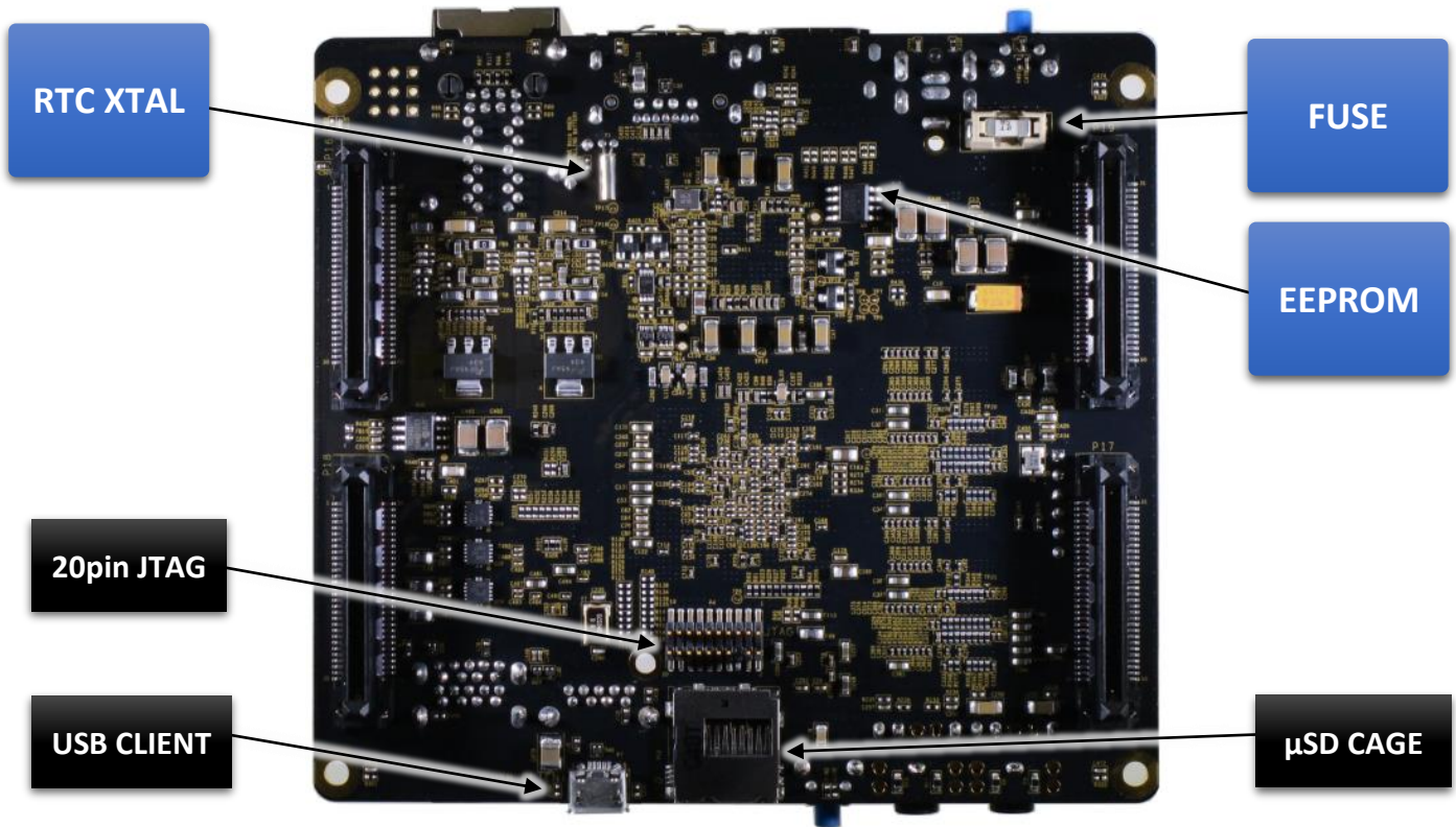
Figure 6. Bottom Side of X15
