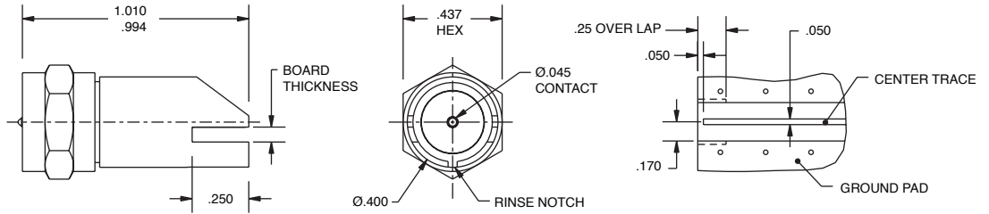
CIRCUIT BOARD EDGE MOUNT "F" STYLE MALE PLUG CBPLE130-1,-2, or -3
