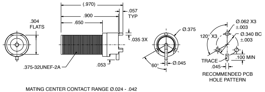
"F" SERIES, BULKHEAD, CIRCUIT BOARD MOUNT RECEPTACLE CBBJ139
