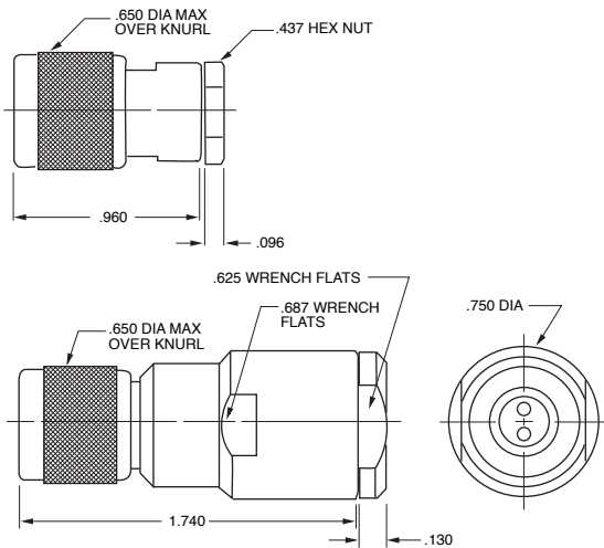
CABLE PLUG TWTNC POSITIVE ALIGNING TWO-PIN POLARIZED
