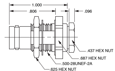
BULKHEAD CABLE JACK REAR MOUNT, WRENCH CRIMP TWO-PIN POLARIZED
