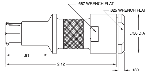
PATCH PLUG 50Ω-WITHOUT LOCKING SLEEVE
