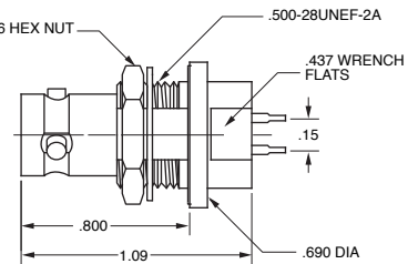
HERMETICALLY SEALED MINIATURE TWINAX/TRIAX FEED-THRU BULKHEAD MOUNT Mounting Hole: D3.187 BJ78HS BJ378HS (Threaded Version Not Shown) INSULATED VERSION BJ73HS (Not Shown) Mounting Hole: D2.187
