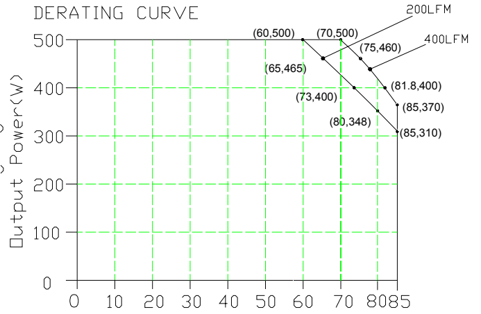
AMBIENT TEMPERATURE, T_a (°C) Output Power vs. Local Ambient Temperature and Air Velocity
