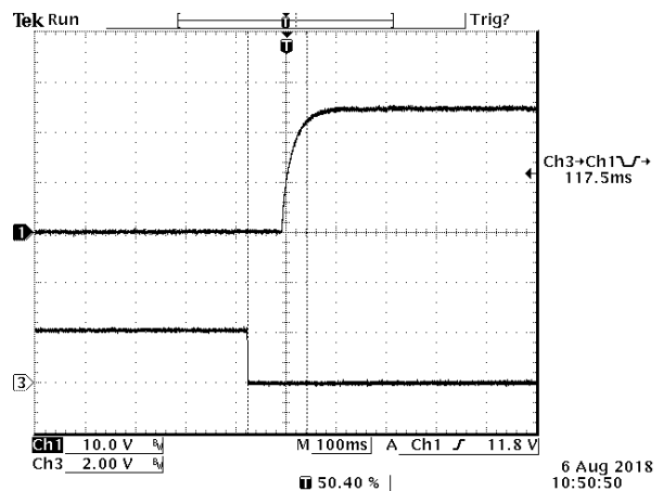
Figure 33. Startup from on/off Ch1: Vo Ch3: Vin
