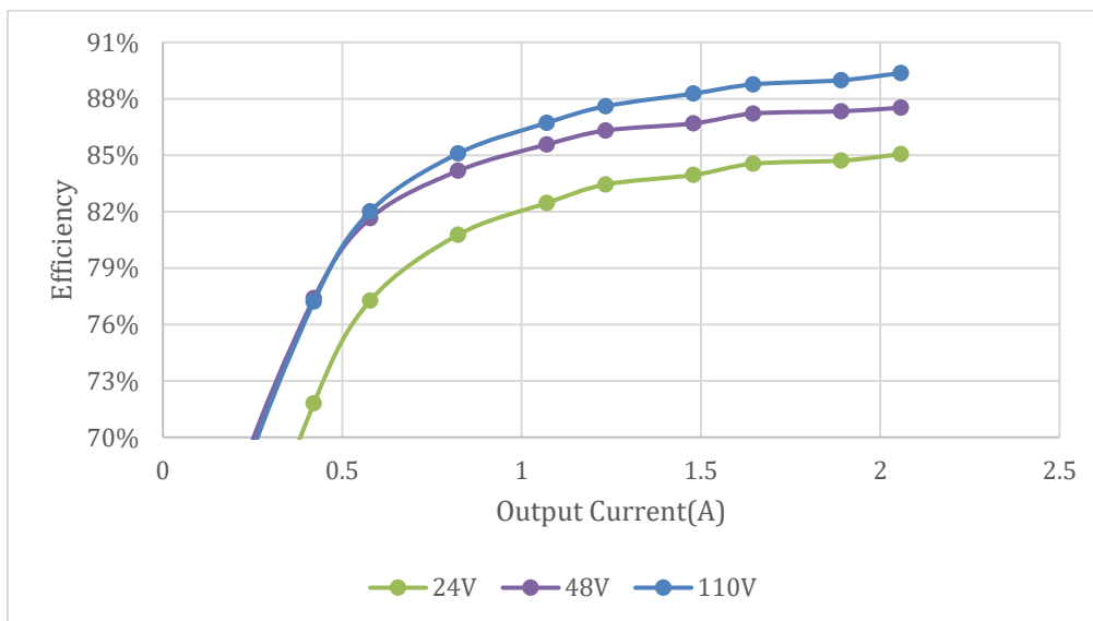
Figure 1. Efficiency data
