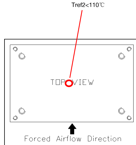
Figure 27. Temperature reference points on top side
