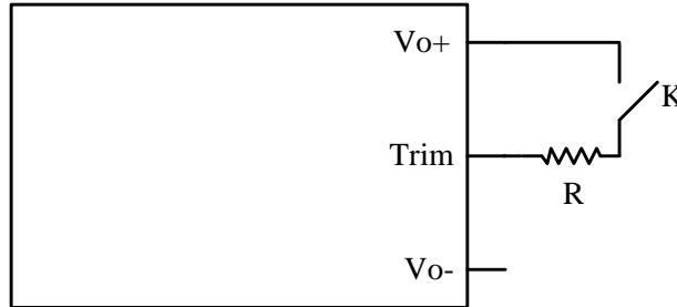
Figure 25. Test setup
