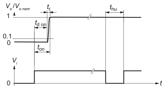
Fig. 8b Typical output response to V_i if option M is not fitted, t_{hu} = 0 ms.
