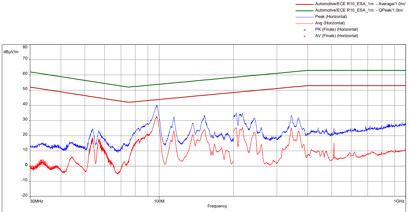
Fig. 10 12RCM60-24: Typ. radiated disturbances in 1 m distance ( V_i = 13.5 \text{ V} , I_{i_{nom}} resistive load, peak & average)
