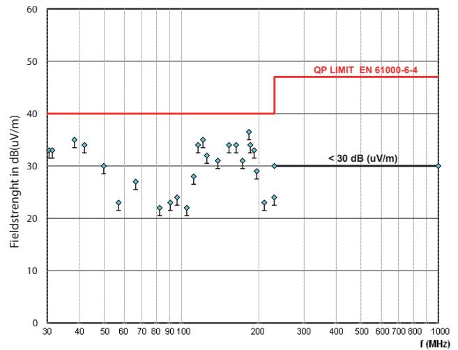
Fig. 9b XRCM60-24: Typ. radiated disturbances in 10 m distance ( V_i = 137.5 \text{ V} , I_{i \text{ nom}} , resistive load, quasi peak).
