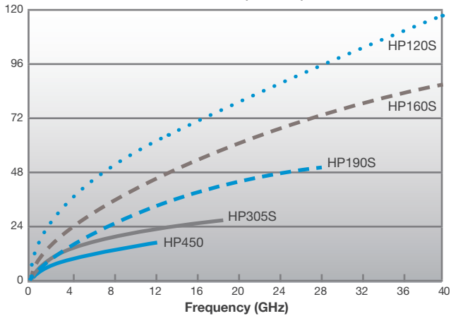
Attenuation* (dB/100ft)
