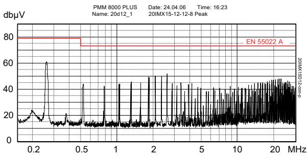
Fig. 17a 20IMX15-12-12-8: Typ. disturbance voltage (peak) at pos. input according to EN 55011, measured at V_{i\text{nom}} and I_{o\text{nom}} .
