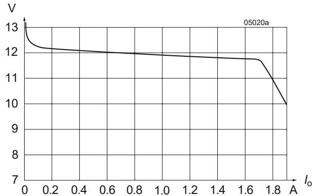
Fig. 10 V_o versus I_o (typ.) of double-output models (2 x 12 V), with both outputs in parallel (110IMY15-12-12-8)
