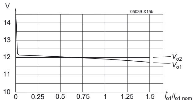
Fig. 12 Flexible load distribution on double-outputs models with option R (110IMY15-12-12-8R): Load variation from 0 to 150% of I_{o1\text{ nom}} on output 1; output 2 loaded with 50% of I_{o2\text{ nom}}
