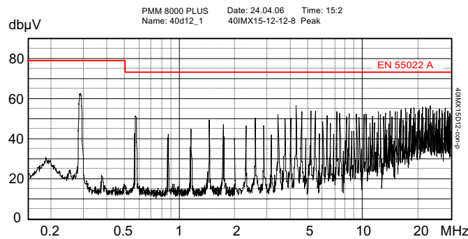
Fig. 18 Typ. disturbance voltage (peak) at input according to EN 55011/022, measured at V_{i\text{nom}} and I_{o\text{nom}} . Output leads 0.1 m, twisted, input filter as in fig. 19 (40IMX15-12-12-8)
