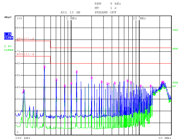
Fig. 14 Typ disturbances (quasi-peak and average) at the input according to EN 50121-4, measured at V_{i\text{nom}} and I_{o\text{nom}} (110IMX35D05D15-8).
