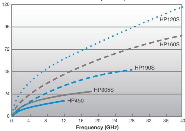
Attenuation* (dB/100ft)
