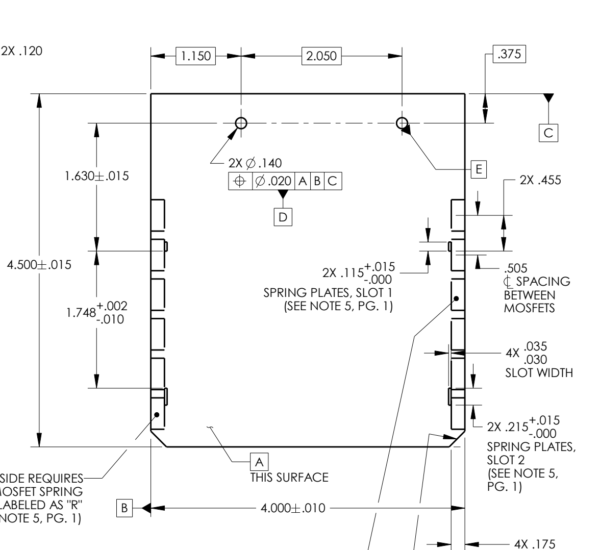
PCB OVERALL DIMENSIONS AND HOLE LOCATIONS
