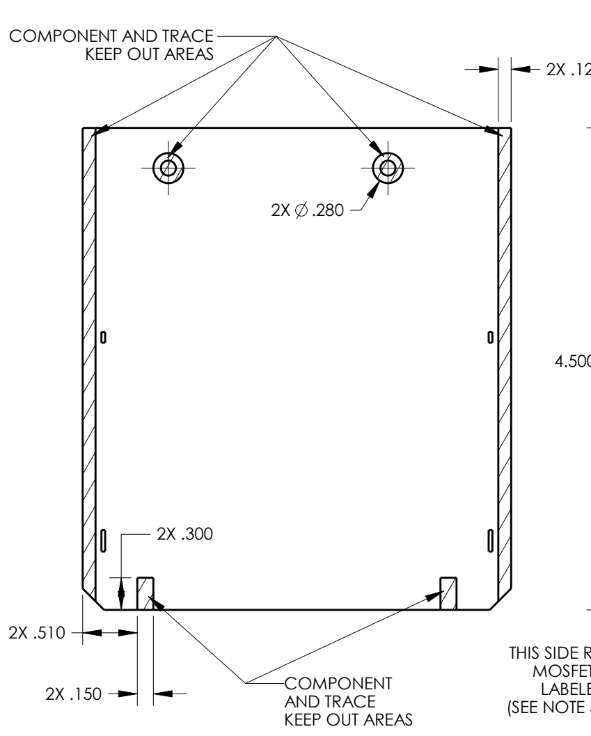
PCB BOTTOM SIDE GENERAL ZONING & KEEP OUT AREAS
