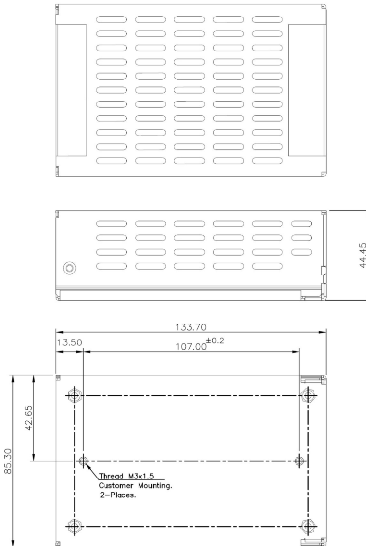
MECHANICAL OUTLINE DIMENSIONS ALL DIMENSIONS ARE IN MM. GEN. TOLERANCE: ±1.0 mm
