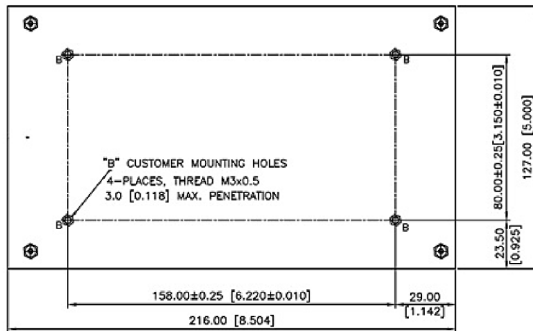
BOTTOM VIEW
