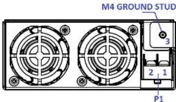
Figure 8. Front View - ABE1200-1T24 / ABE1200-1T48 Models
