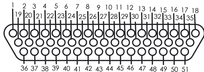
51 CONTACTS
