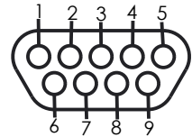
9 CONTACTS
