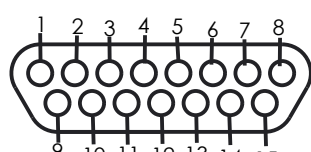
15 CONTACTS
