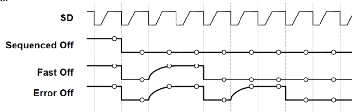
Figure 35. OK Severity Encoding Waveforms
