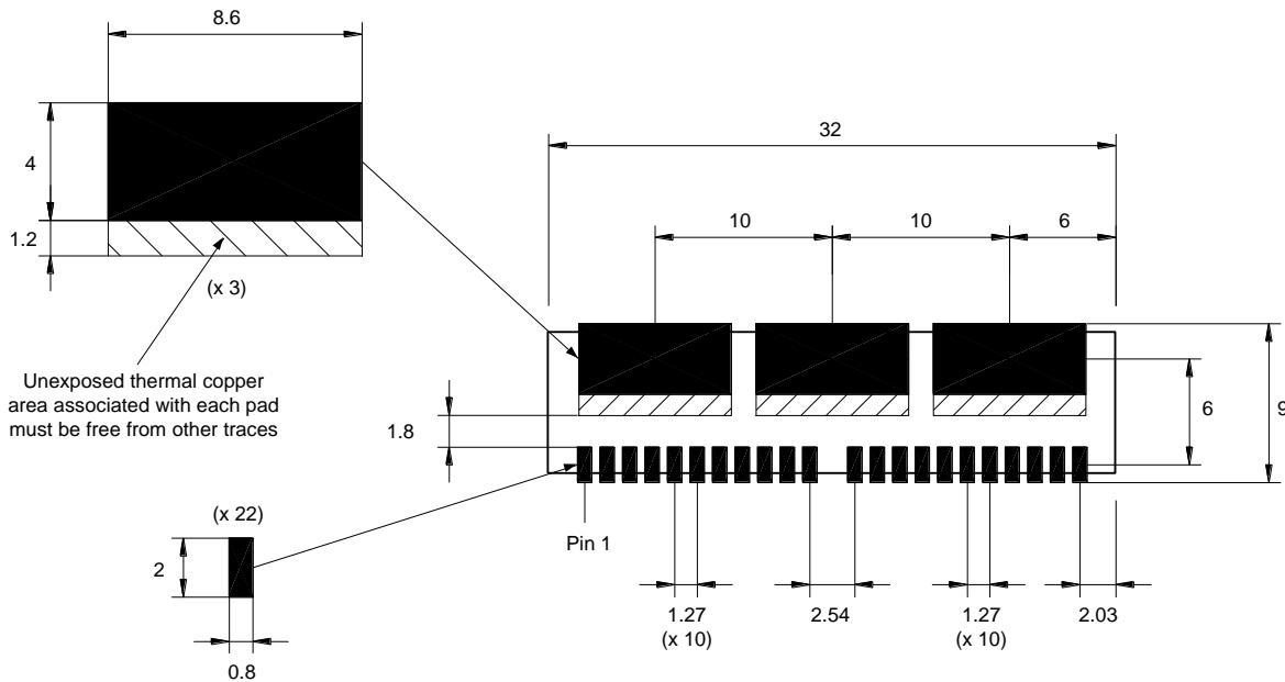
Figure 60. Recommended Pad Sizes
