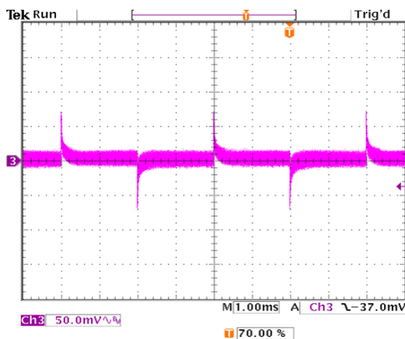
Figure 50. Transient Response with Regulation set to 0.0 mV/A.
