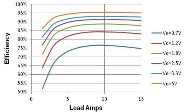
Figure 8 Efficiency vs Load. V_{in}=8V , F_{sw}=1MHz
