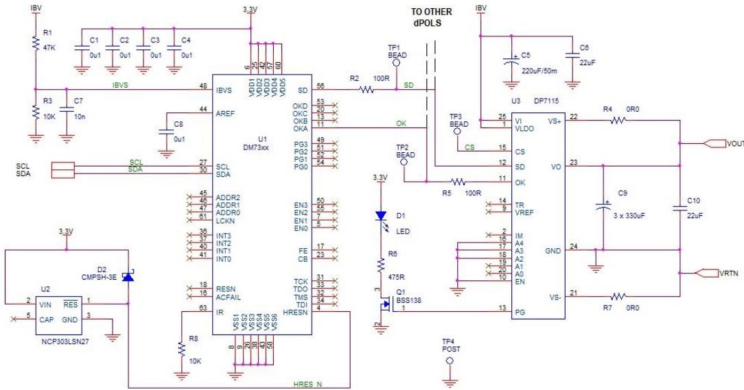
Figure 57. Typical Application with Digital Power Manager and I2C Interface
