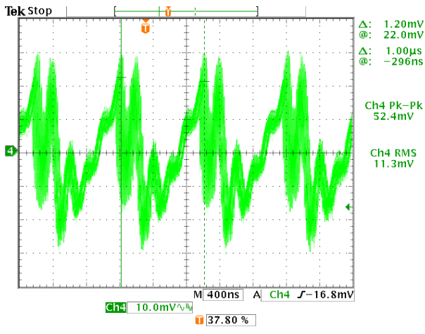
Figure 45. Input Voltage Noise, No Interleave
