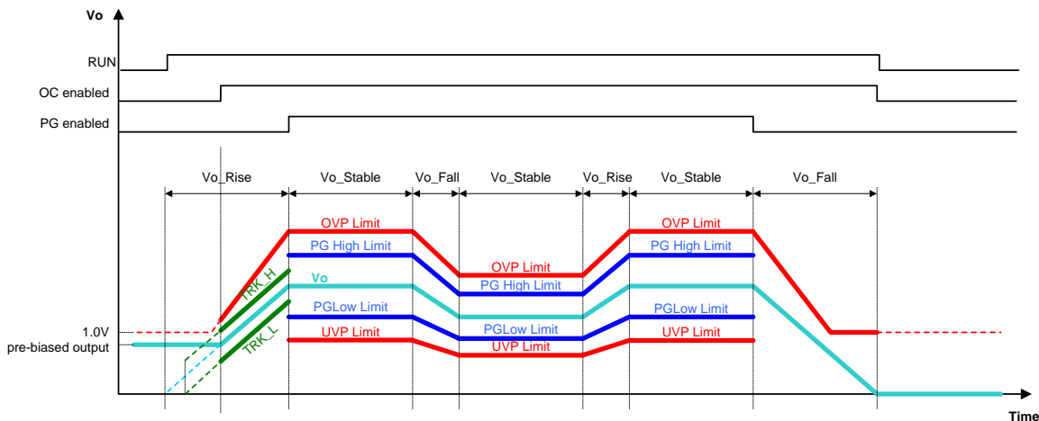
Figure 32. Protection Enable Conditions
