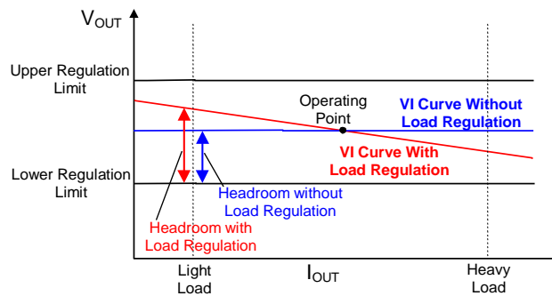
Figure 15. Optimal Voltage Positioning Concept
