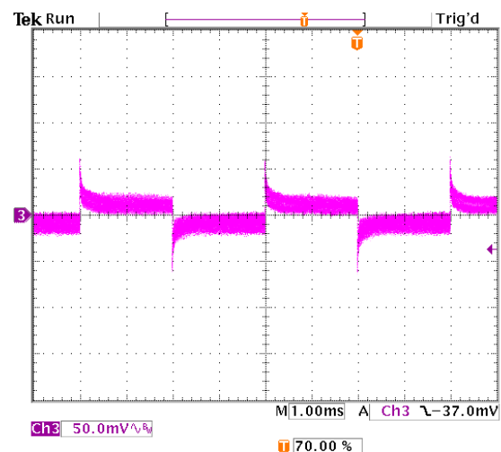
Figure 51. Transient Response with Regulation set to 3.72 mV/A.
