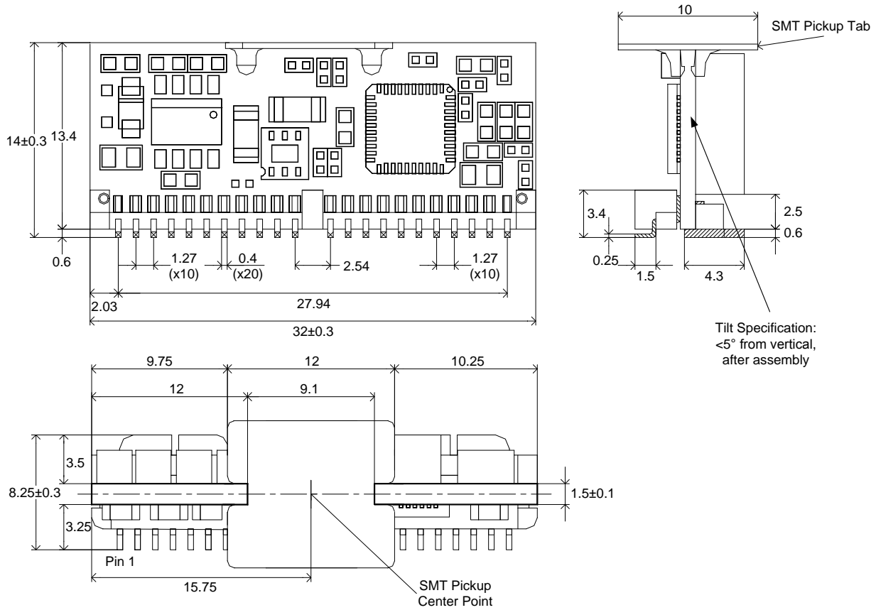
Figure 58 Mechanical Drawing
