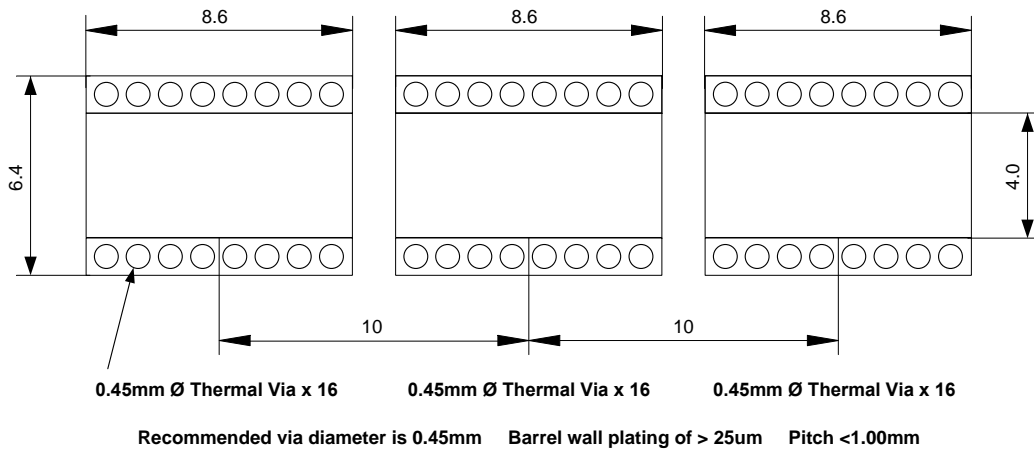
Figure 61. Recommended PCB Power Tab (Pins 23 - 25) Layout for Multilayer PCBs
