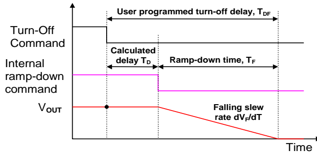
Figure 22. Relationship between Turn-Off Delay and Falling Slew Rate
