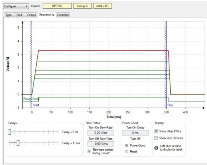
Figure 20. dPOL Configure Sequencing Window
