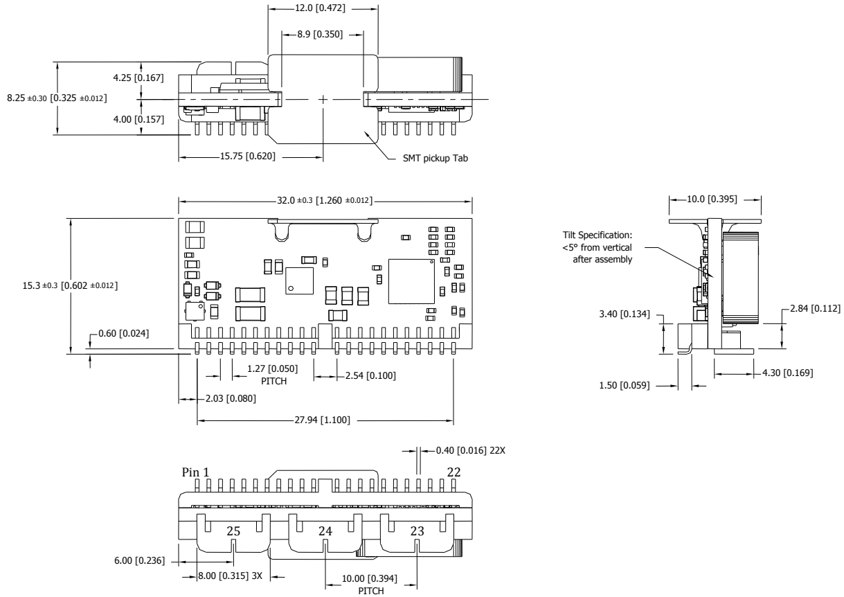
Figure 55: Mechanical Drawing
