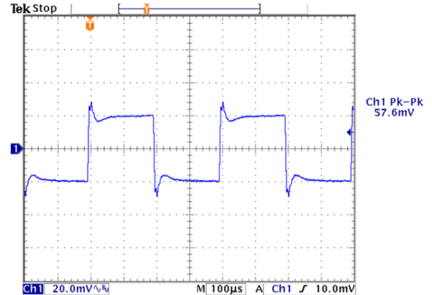
Figure 14. Transient Response with non-zero Regulation.
