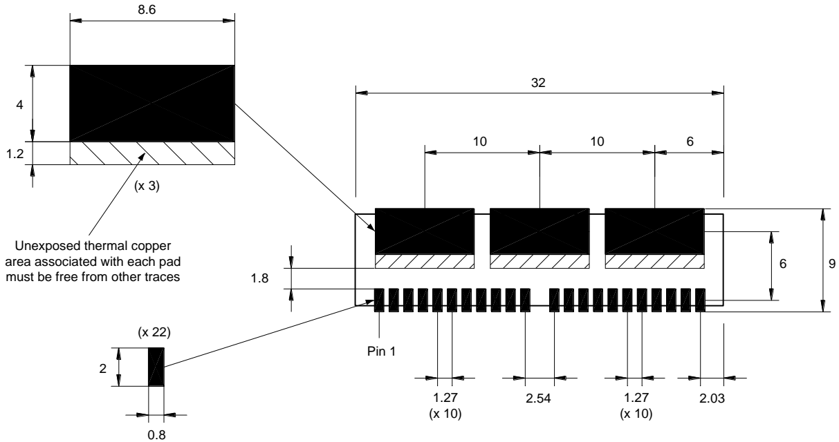
Figure 57: Recommended Pad Sizes
