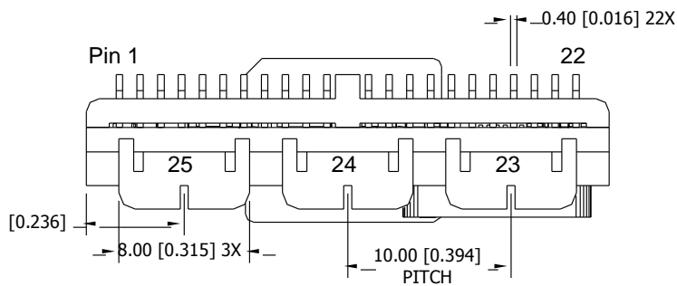
Figure 56: Pinout Diagram (Bottom View)
