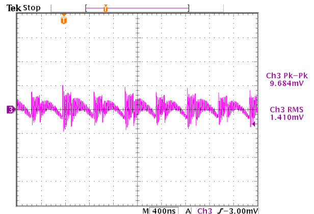
Figure 45. Output Voltage Noise, Full Load, 180° Interleave
