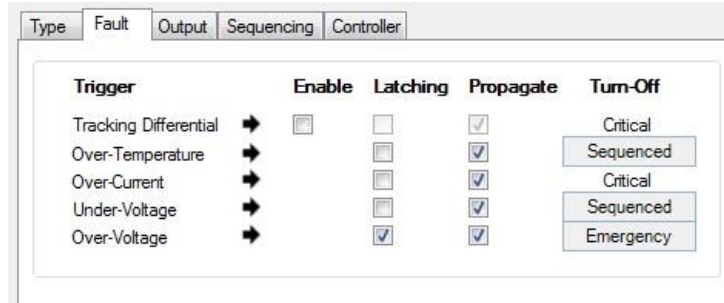
Figure 31. GUI dPOL Fault Latching and Propagation Option Window
