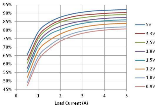
Figure 3. Efficiency vs. Load, V_{in}=12\text{V} , F_{sw}=500\text{KHz}
