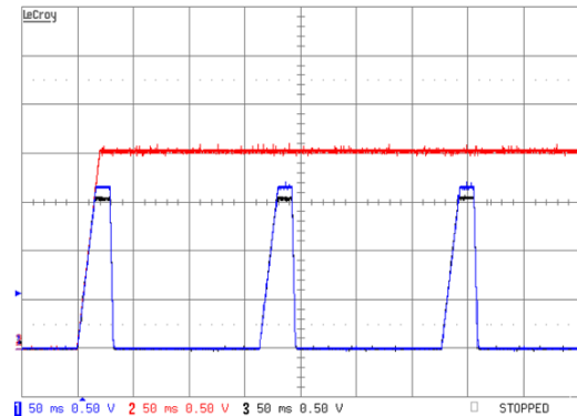
Figure 34. Turn-On into UVP on V3. The UV Fault is programmed to be Non-Latching and Propagate From Group C to Group A. Ch1 - V3(Group c), Ch2 - V2, Ch3 - V1 (Group A)
