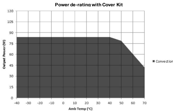
Figure 1. Derating Curves
