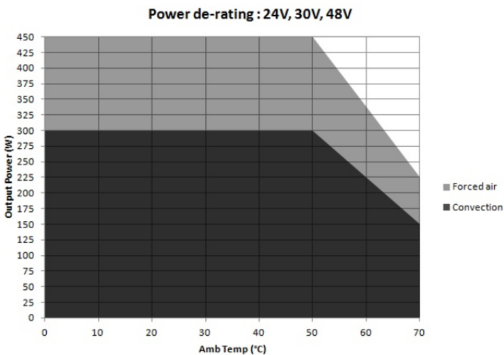
Figure 1. Derating Curves
