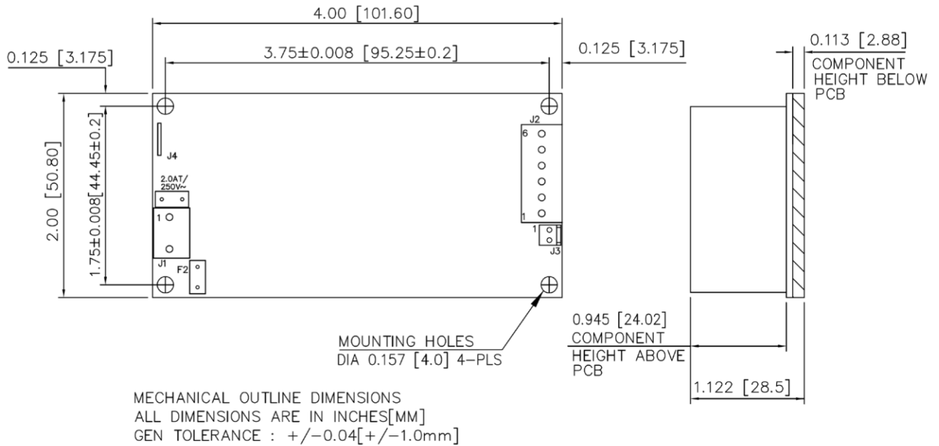
Figure 3. Mechanical Drawing MBC60-1xxxG
