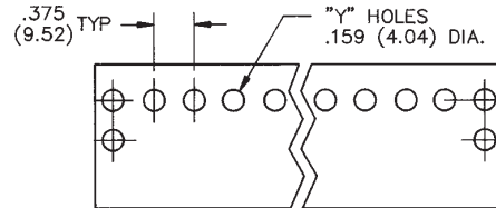
"Y" Terminal
