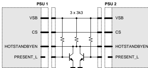
Figure 31. Recommended hot-standby configuration
