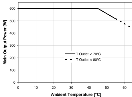
Figure 39. Thermal derating for PFE600-12-054NA
