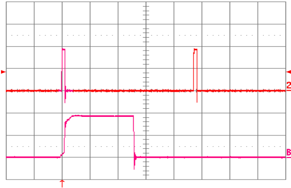
Figure 25. Load current (top trace, 20 A/div, 20 ms/div) into a 10 mΩ short circuit during restart, at V_{in} = 24\text{ V} . Bottom trace (20 A/div, 1 ms/div) is an expansion of the on-time portion of the top trace.
