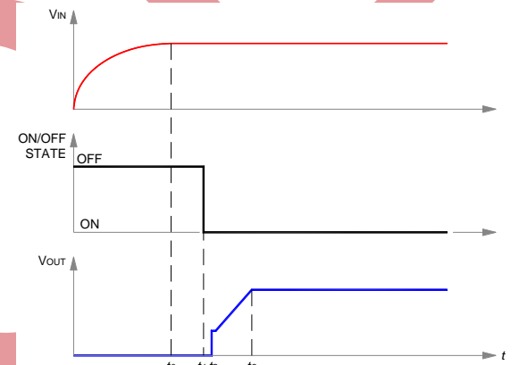
Figure 6. Startup scenario #2.
