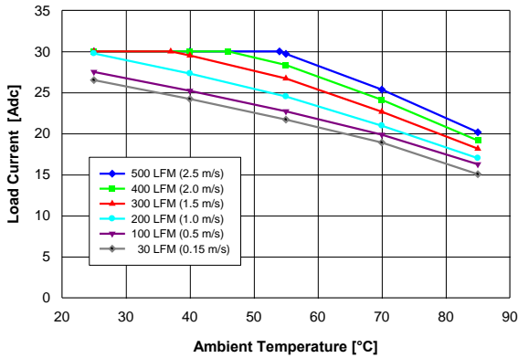
Figure 10. Available load current vs. ambient temperature and airflow rates for converter mounted horizontally with V_{in} = 27\text{ V} , air flowing from pin 3 to pin 4 and maximum FET temperature \leq 120\text{ }^{\circ}\text{C} .
