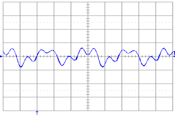
Figure 20. Output voltage ripple (20 mV/div.) at full rated load current into a resistive load with C_o = 10 F tantalum + 1 \mu F ceramic and V_{in} = 24 V. Time scale: 1 \mu s/div..
