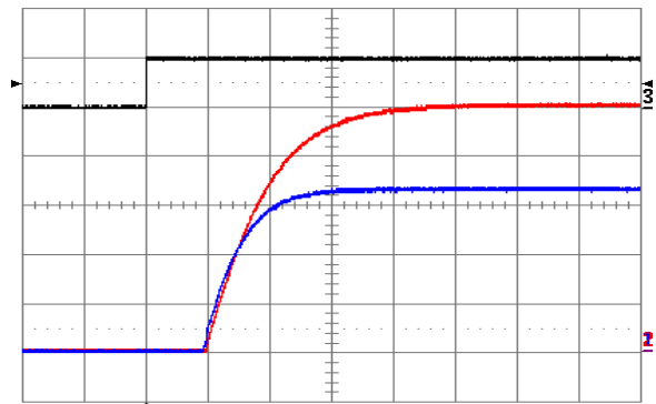
Figure 22. Turn-on transient waveforms at full rated load current (resistive) and V_{in} = 48 V, triggered via ON/OFF pin. Top trace: ON/OFF signal (5 V/div.). Bottom traces: V_{out1} (blue, 1 V/div.), V_{out2} (red, 1 V/div.). Time scale: 1 ms/div.
