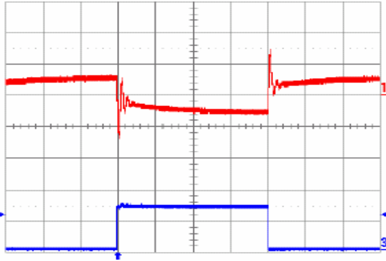
Fig. 13: Step Load response to 0% – 50% – 0% with 100 \mu F external ceramic capacitor and di/dt = 10 \text{ A}/\mu\text{s} . Top trace: output voltage (500 mV/div.). Bottom trace: load current (10 A/div). Time scale: 0.2 ms/div.
