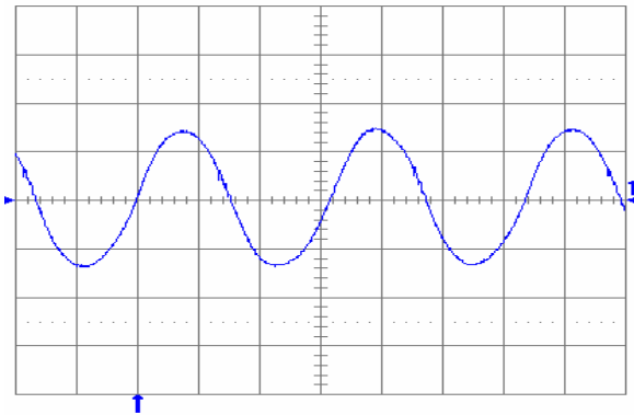
Fig. 15: Output voltage ripple (50 mV/div.) at full rated load current into a resistive load with C_o = 10 \mu\text{F} tantalum + 1 \mu\text{F} ceramic and V_{in} = 56 \text{ V} . Time scale: 1 \mu\text{s}/\text{div} .
