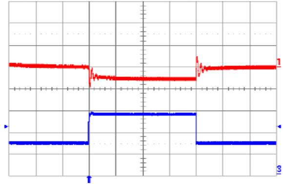
Fig. 14: Step Load response to 50% – 100% – 50% with 100 \mu F external ceramic capacitor and di/dt = 10 \text{ A}/\mu\text{s} . Top trace: output voltage (500 mV/div.). Bottom trace: load current (5 A/div). Time scale: 0.2 ms/div.
