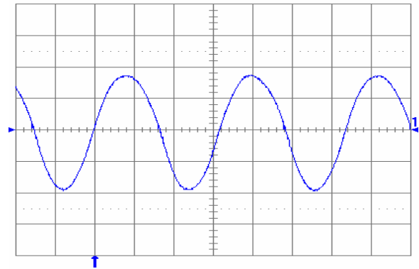
Fig. 16: Output voltage ripple (50 mV/div.) at full rated load current into a resistive load with C_o = 10 \mu\text{F} tantalum + 1 \mu\text{F} ceramic and V_{in} = 75 \text{ V} . Time scale: 1 \mu\text{s}/\text{div} .
