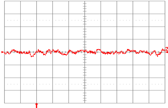
Fig. 1.5V.12: Input reflected ripple current, i_s (10 mA/div), measured through 10 \mu\text{H} at the source at full rated load current and V_{in} = 48 \text{ V} . Refer to Fig. 1.5V.11 for test setup. Time scale: 1 \mu\text{s}/\text{div} .
