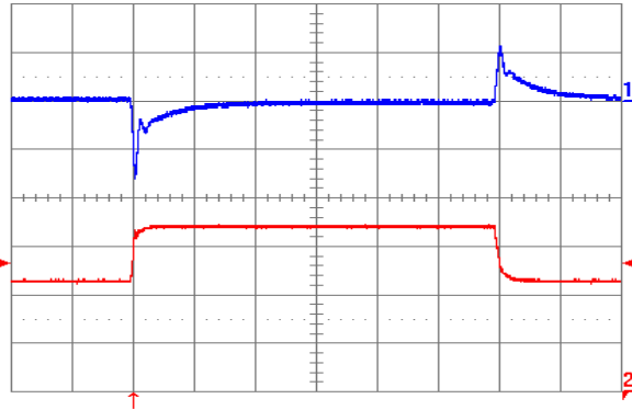
Fig. 1.8V.9: Output voltage response to load current step-change (22.5 A – 33.75 A – 22.5 A) at V_{in} = 48 V. Top trace: output voltage (20 mV/div.). Bottom trace: load current (10 A/div.). Current slew rate: 1 A/ \mu s. C_o = 470 \mu F tantalum + 1 \mu F ceramic. Time scale: 0.2 ms/div.
