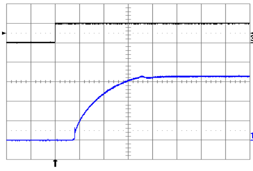
Fig. 3.3V.8: Turn-on transient at full rated load current (resistive) plus 40,000 \mu\text{F} at V_{in} = 48\text{ V} , triggered via ON/OFF pin. Top trace: ON/OFF signal (5 V/div.). Bottom trace: output voltage (1 V/div.) Time scale: 2 ms/div.
