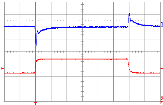
Fig. 1.5V.9: Output voltage response to load current step-change (22.5 A – 33.75 A – 22.5 A) at V_{in} = 48\text{ V} . Top trace: output voltage (100 mV/div.). Bottom trace: load current (10 A/div). Current slew rate: 1 A/ \mu\text{s} . C_o = 470\text{ }\mu\text{F} tantalum + 1 \mu\text{F} ceramic. Time scale: 0.2 ms/div.
