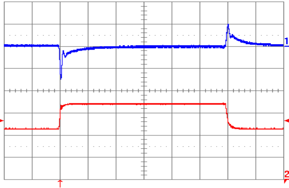
Fig. 2.0V.9: Output voltage response to load current step-change (22.5 A - 33.75 A - 22.5 A) at V_{in} = 48\text{ V} . Top trace: output voltage (100 mV/div.). Bottom trace: load current (10 A/div). Current slew rate: 1 A/ \mu\text{s} . C_o = 470\text{ }\mu\text{F} tantalum + 1 \mu\text{F} ceramic. Time scale: 0.2 ms/div.
