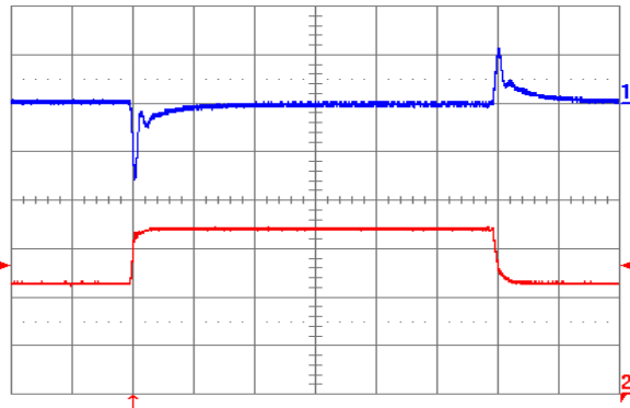
Fig. 1.0V.9: Output voltage response to load current step-change (22.5 A – 33.75 A – 22.5 A) at V_{in} = 48\text{ V} . Top trace: output voltage (100 mV/div.). Bottom trace: load current (10 A/div). Current slew rate: 1 A/ \mu\text{s} . C_o = 470\text{ }\mu\text{F} tantalum + 1 \mu\text{F} ceramic. Time scale: 0.2 ms/div.
