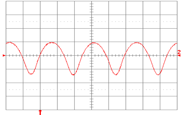
Fig. 1.0V.13: Input reflected ripple current, i_c (100 mA/div), measured at input terminals at full rated load current and V_{in} = 48\ \text{V} . Refer to Fig. 1.0V.11 for test setup. Time scale: 1\ \mu\text{s}/\text{div} .
