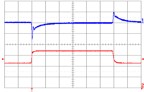
Fig. 3.3V.9: Output voltage response to load current step-change (22.5 A – 33.75 A – 22.5 A) at V_{in} = 48 V. Top trace: output voltage (100 mV/div.). Bottom trace: load current (10 A/div.). Current slew rate: 1 A/ \mu s. C_o = 470 \mu F tantalum + 1 \mu F ceramic. Time scale: 0.2 ms/div.
