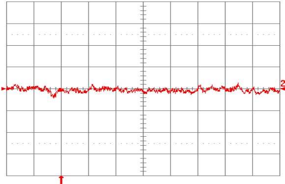
Fig. 1.0V.12: Input reflected ripple current, i_s (10 mA/div), measured through 10\ \mu\text{H} at the source at full rated load current and V_{in} = 48\ \text{V} . Refer to Fig. 1.0V.11 for test setup. Time scale: 1\ \mu\text{s}/\text{div} .
