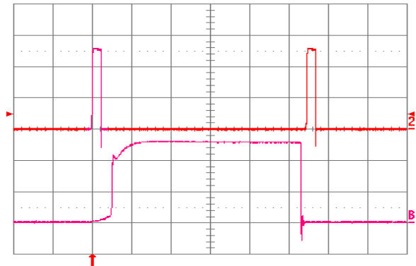
Fig. 1.0V.15: Load current (top trace, 20\ \text{A}/\text{div} , 20\ \text{ms}/\text{div} ) into a 10\ \text{m}\Omega short circuit during restart, at V_{in} = 48\ \text{V} . Bottom trace ( 20\ \text{A}/\text{div} , 1\ \text{ms}/\text{div} ) is an expansion of the on-time portion of the top trace.
