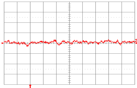
Fig. 1.2V.12: Input reflected ripple current, i_s (10 mA/div), measured through 10 \mu H at the source at full rated load current and V_{in} = 48 V. Refer to Fig. 1.2V.11 for test setup. Time scale: 1 \mu s/div.
