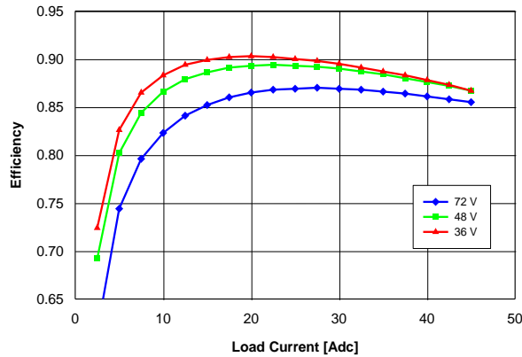
Fig. 1.8V.3: Efficiency vs. load current and input voltage for converter mounted vertically with air flowing from pin 3 to pin 1 at a rate of 300 LFM (1.5 m/s) and T_a = 25\text{ }^\circ\text{C} .
