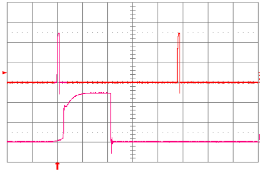
Fig. 2.5V.15: Load current (top trace, 20 A/div, 20 ms/div) into a 10 m \Omega short circuit during restart, at V_{in} = 48 V. Bottom trace (20 A/div, 1 ms/div) is an expansion of the on-time portion of the top trace.
