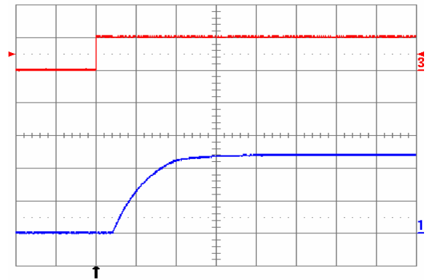
Fig. 8: Turn-on transient at full rated load current (resistive) plus 2,200 µF at V_{in} = 48\text{ V} , triggered via ON/OFF pin. Top trace: ON/OFF signal (5 V/div.). Bottom trace: output voltage (5 V/div.). Time scale: 2 ms/div.
