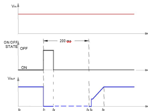
Figure 4. Startup scenario #3.
