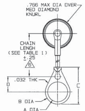
RFI85/RFI853-12-01 THRU -17-008 SHOWN SST ROPE AND BULKHEAD JACK MOUNTING LUG
